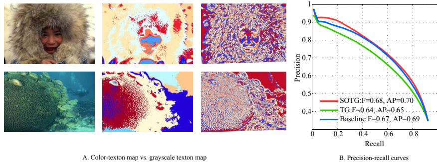
Fig. 4. Contour detection on BSDS500. (A) Some representative examples of tex-ton maps and color extensions. From left to right: original images, color-texton map (SOTG) and tex-ton map (TG). (B) Precision-recall curves on BSDS500, comparing the original grayscale texture channel with the full Berkeley system that combines brightness, color, and texture cues against our color-texture cue.
